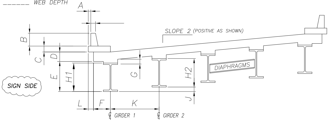
BRIDGE CROSS SECTION
